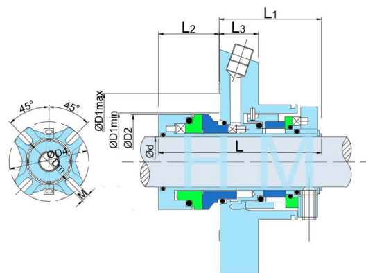
HMCS-B10(CARTEX ANSI-S)-B (use cast cover)
