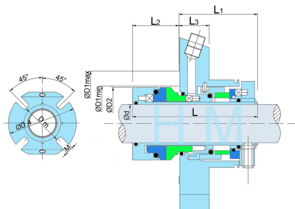
HMCS-B10(CARTEX ANSI-S)-A (Use mechined cover)
