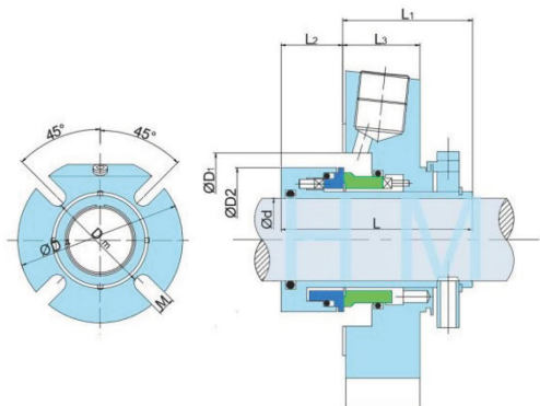
HMCS-B08(CARTEX-SN)-A (use Mechined cover)
