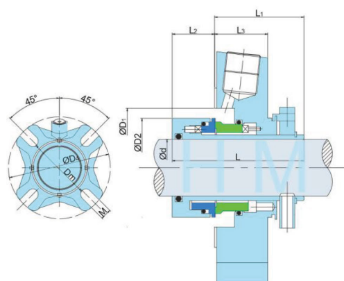
HMCS-B08(CARTEX-SN)-B (use cast cover)
